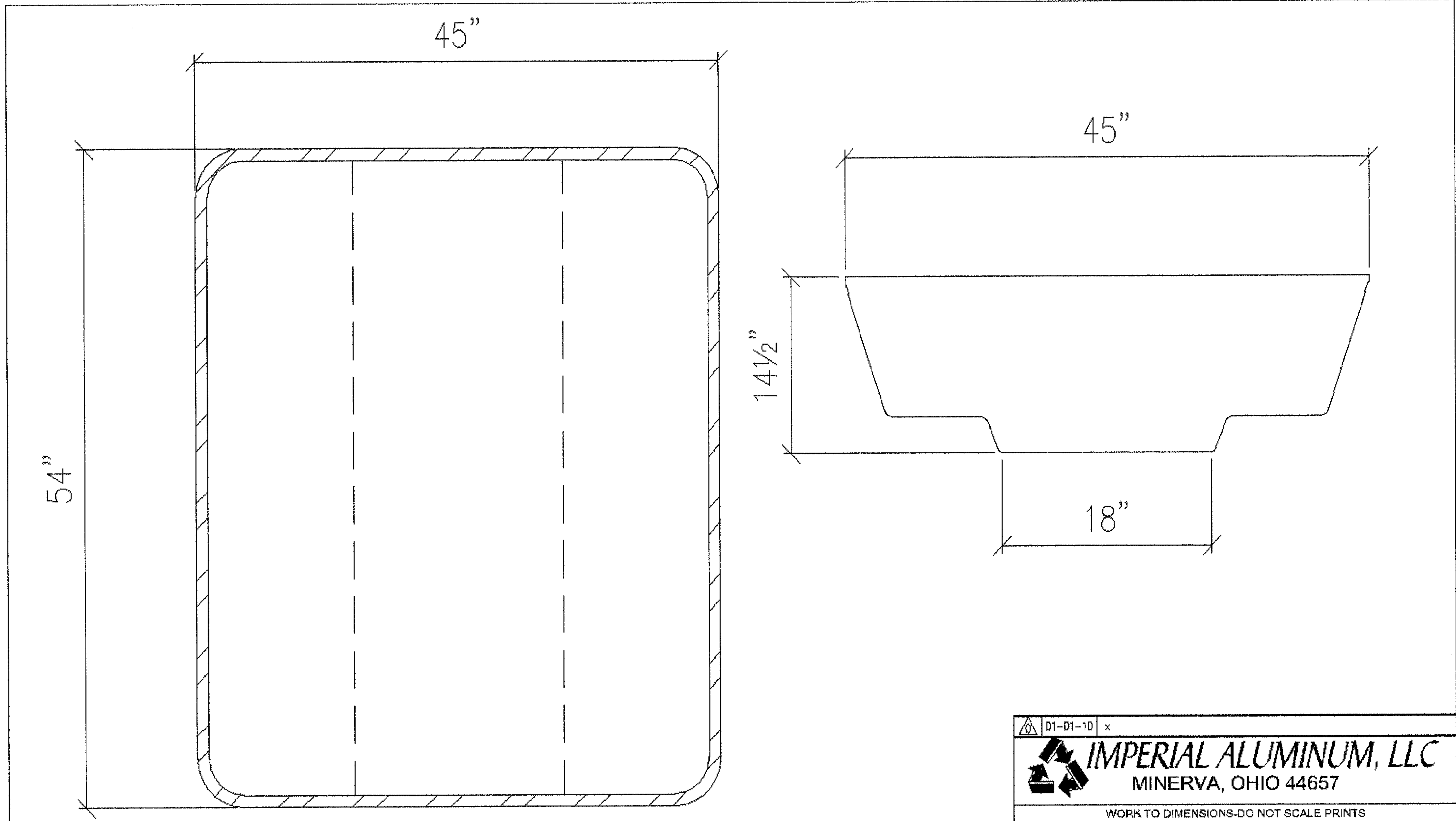
DIMENSIONS OF 1000Kg LOW PROFILE SOW 2,000Lbs
